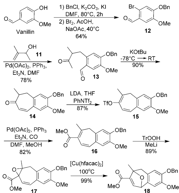
Scheme 2. Synthesis of the functionalized aryl-fused oxatropane. DMF = N,N -dimethylformamide, LDA = lithium diisopropylamide, Tf = trifluorosulfonyl, Tr = triphenylmethyl, hfacac = hexafluoroacetyl acetate.
