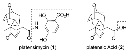
Figure 1. The structures of platensimycin and platensic acid.
